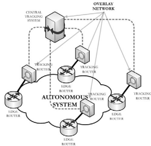
Figure 4 – A simplified version of CenterTrack
